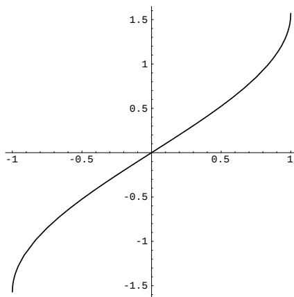
Figure 5.25: \arcsin on [-1, 1]
