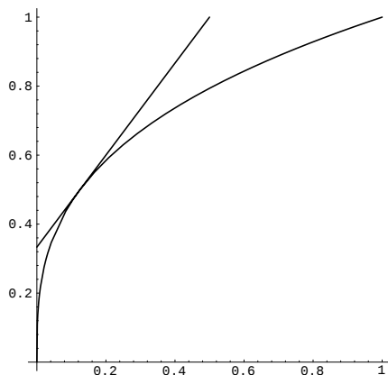
Figure 2.23: g(x) = x^{1/3}
