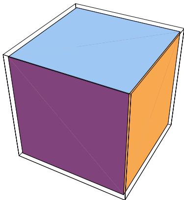
Figure 2.13: A cube
